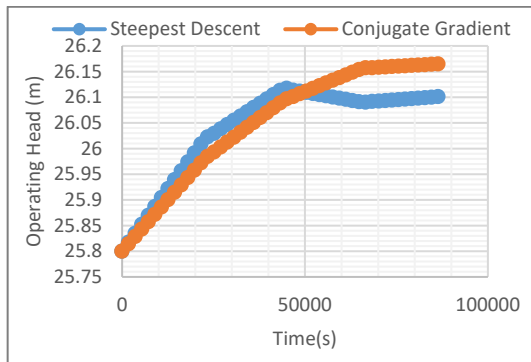
Fig. 14. Comparison of the operating Head by Steepest Descent and Conjugate Gradient Technique for (4, 25.8, 1, u_{max} = 4000 \text{ m}^3/\text{s} )
