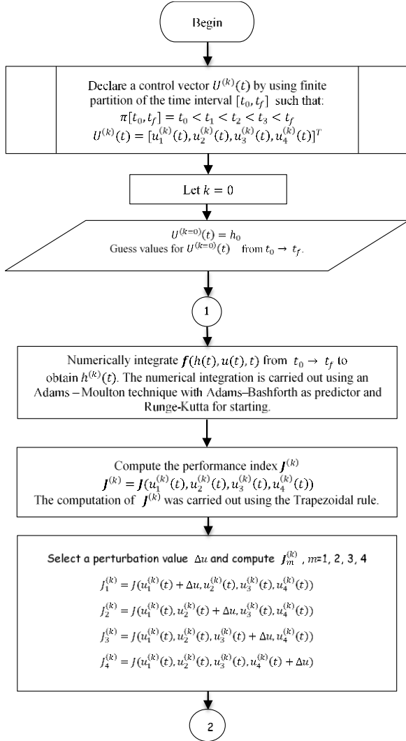
Fig. 4." Flow chart for the direct optimal control of the JHEPS
