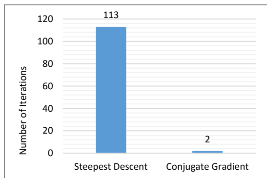
Fig. 15. Comparison of the optimal control by Steepest Descent and Conjugate Gradient Technique for (4, 25.8, 1, u_{max} = 4000 \text{ m}^3/\text{s} )
