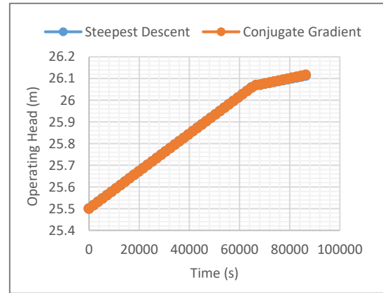
Fig. 11." Comparison of the operating Head by Steepest Descent and Conjugate Gradient under (5, 25.5, 1, u_{max} = 4000 m^3/s )
