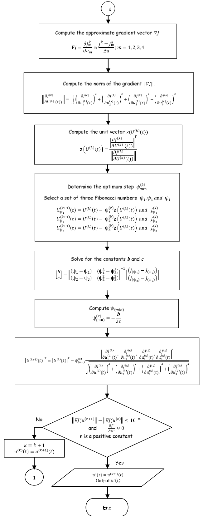
Fig. 5." Flow chart for the Optimal Control By Steepest Descent Algorithm
