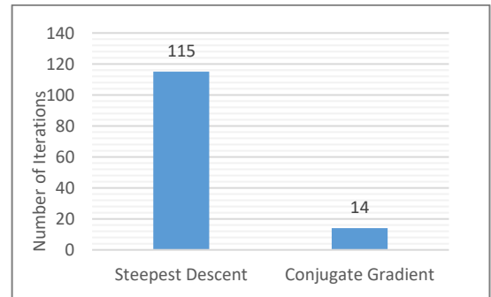
Fig. 13."Number of iterations (5, 25.5, 1, u_{max} = 4000 m^3/s )
