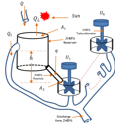
Fig. 3." The structural model of the JHEPS system
