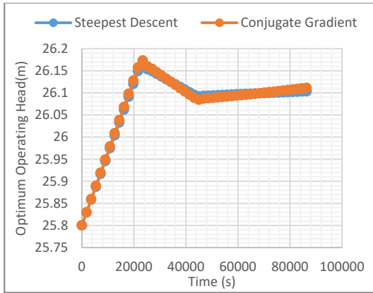
Fig. 8." Comparison of the operating Head by Steepest Descent and Conjugate Gradient under (5, 25.8, 1, u_{max} unpenalized)
