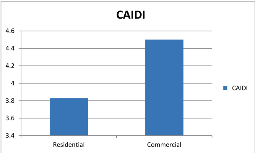
Fig. 9. CAIDI on residential and commercial feeders.
