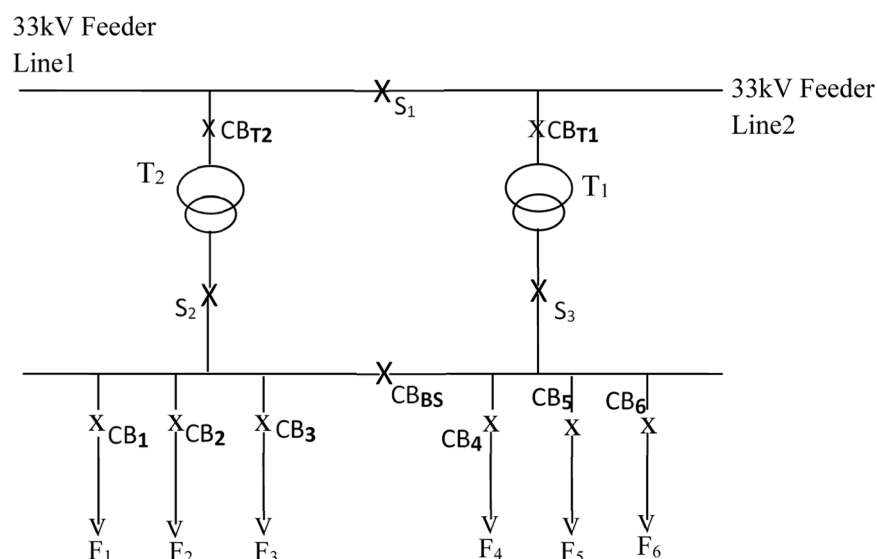
Fig. 1. Agba water work 2 \times 15 MVA, 33/11 kV power injection substation.
