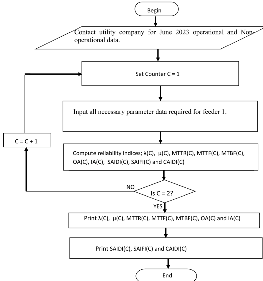
Fig. 2. Flow chart showing the Procedural steps in reliability analysis.
