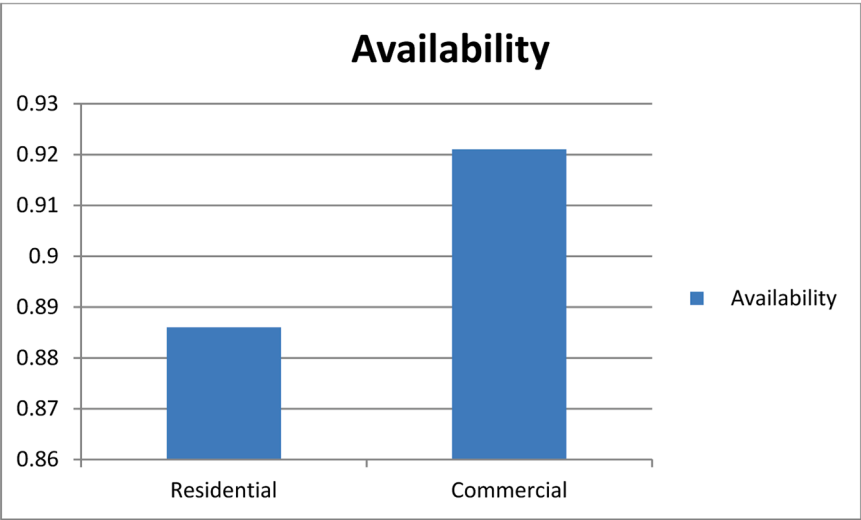
Fig. 5. Availability on residential and commercial feeders.
