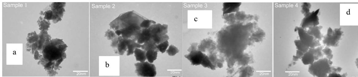
Fig. 3, Transmission electron microscopic images of flamboyant pod particles obtained at (a) 8 charge ratios, 25 hours of milling, (b) 8 charge ratios, 55 hours of milling (c) 10 charge ratios, 25 hours of milling and (d) 10 charge ratios, 55 hours of milling
