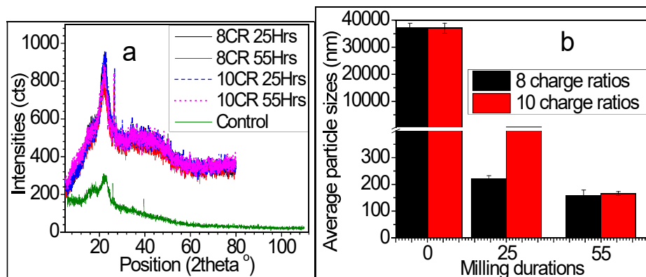
Fig. 2 , (a) superimposed diffractograms of flamboyant pod particles obtained at different milling at 8 and 10 charge ratios by milling for 25 and 55 hours (b) average sizes of the milled flamboyant particles determined using XRD aided with Scherrer's formula
