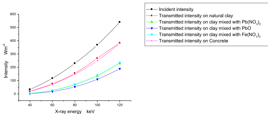
Figure 2: Graph of intensity of natural and artificially contaminated clay against x-ray energy.
