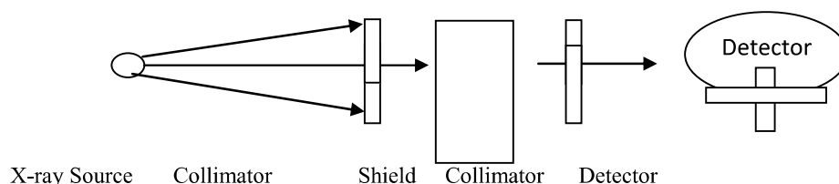
Figure 1: Block diagram of the passage of radiation photon through shield to detector.
