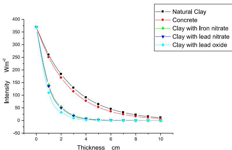
Figure 3: Graph of Intensity against the thickness of concrete, natural and artificially contaminated clay slab at 100keV
