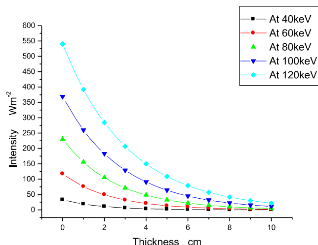
Figure 4: Graph of intensity against thickness of natural clay slabs at different energies.
