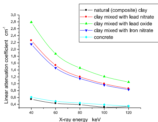
Figure 1: Linear attenuation coefficient of natural and contaminated clay versus x-ray energy for selected shielding types.
