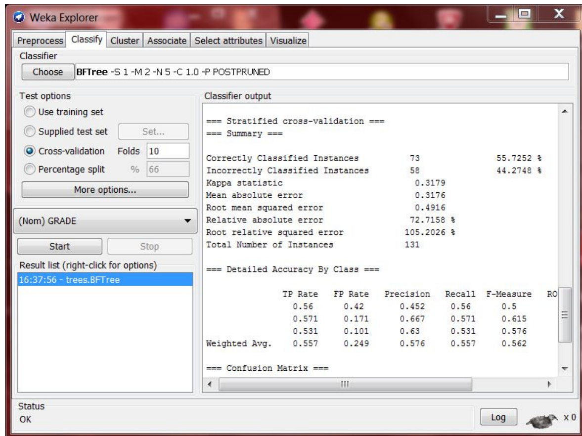
Figure 7: BF Tree Classifier Result
