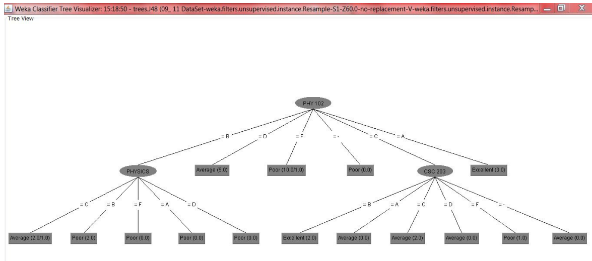
Figure 5: CART Visualization
