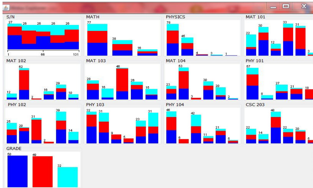
Figure 9: Attributes visualization
