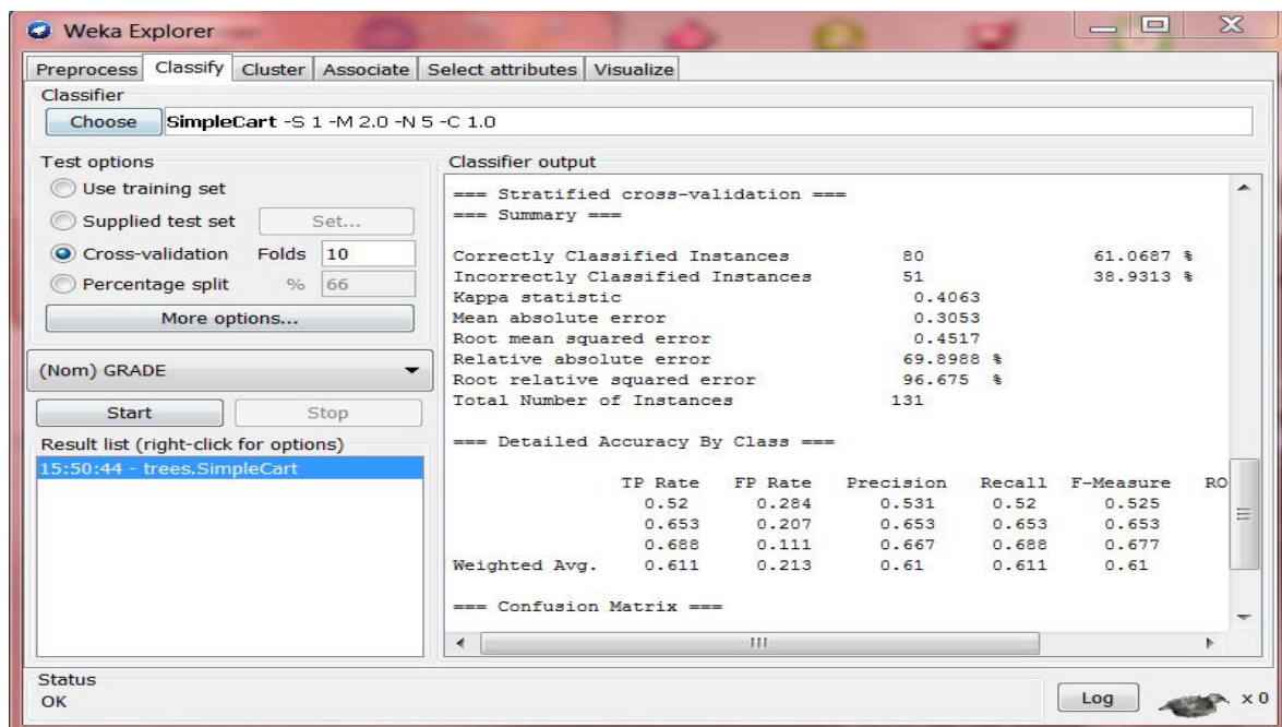
Figure 6: CART Classifier Result
