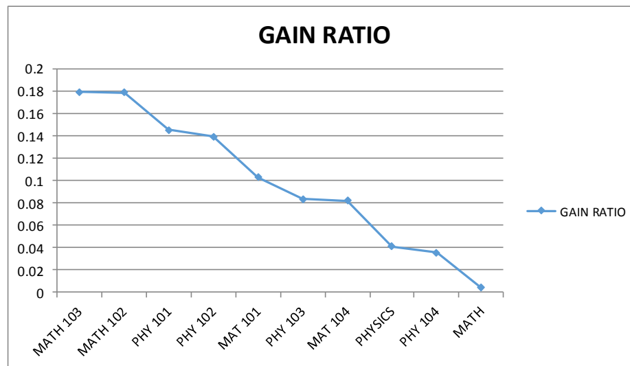
Figure 10: Gain ratio of the attributes
