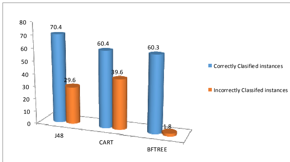
Figure 8: Classification accuracy on 10- folds Cross- validation method
