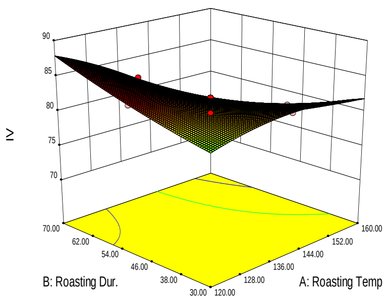
Figure 5. Plot of Iodine Value (IV) against roasting temperature and duration
