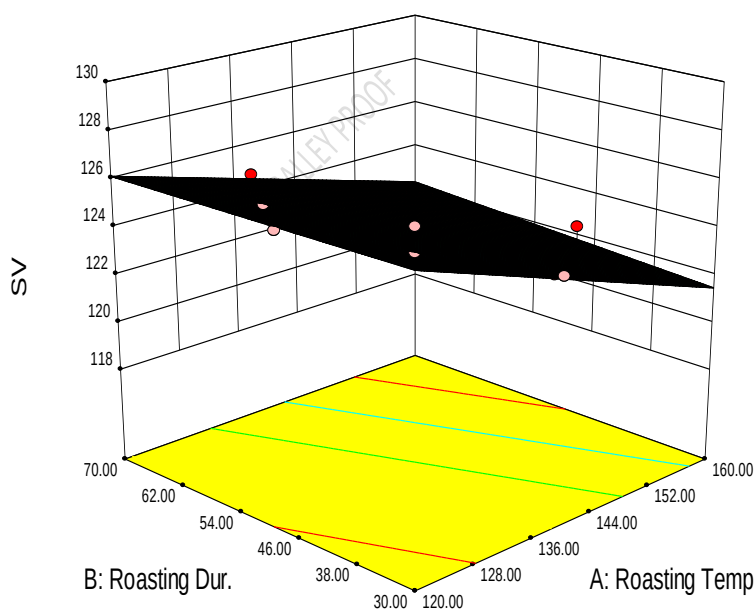
Figure 6: Plot of Saponification Value (SV) against roasting temperature and duration
