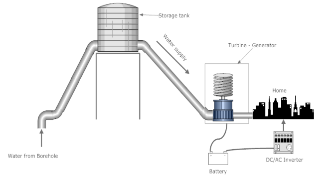
Figure 4: Layout of the proposed system
