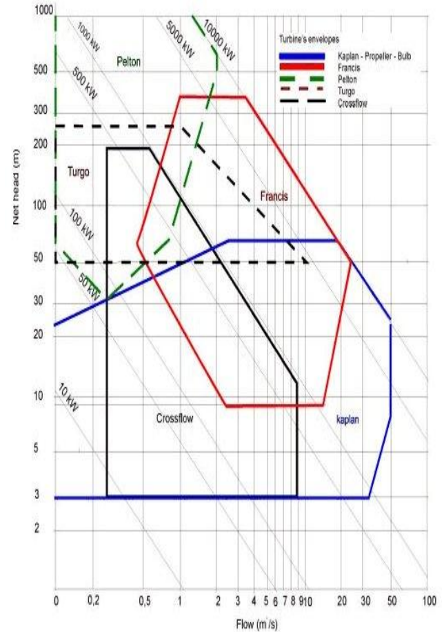
Figure 8: Turbine application range chart
