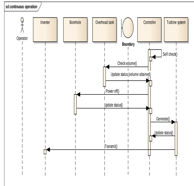
Figure 7: Sequence diagram illustrating the continuous operation of the system
