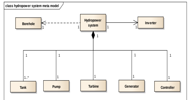
Figure 5: Meta model of the baseline concept
