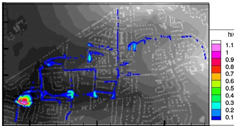
Fig. 1. Flood map of Central model (West Garforth case study area) showing water depth (h).
