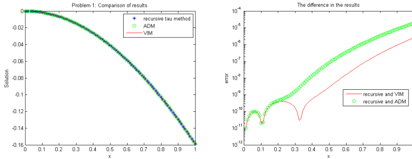
FIGURE 1. Solutions to Problem 1 and their differences
