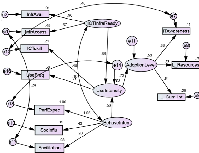
Figure 4 The final model after the third modification (see online version for colours)
