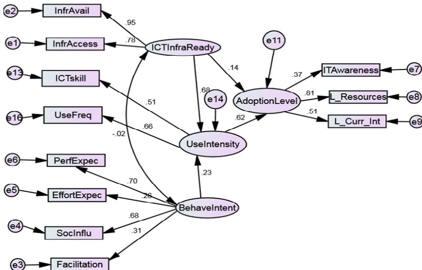
Figure 3 ICT adoption model specification and standard output (see online version for colours)
