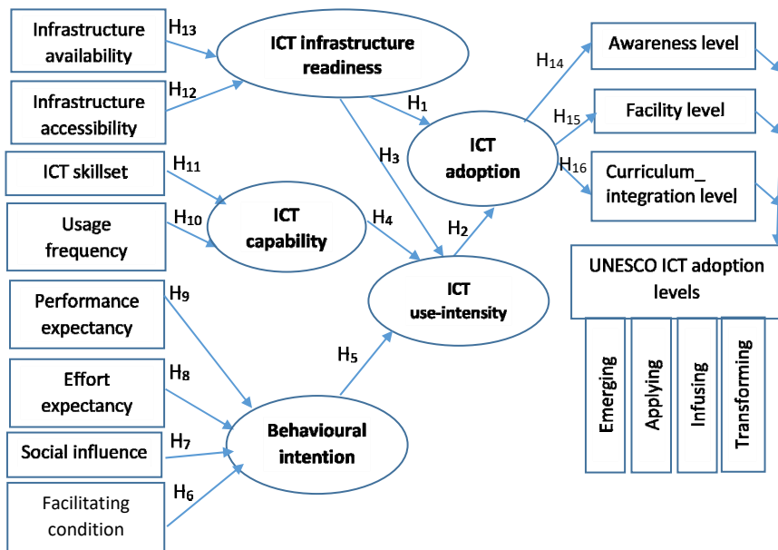
Figure 2 Proposed integrated ICT adoption model (see online version for colours)
