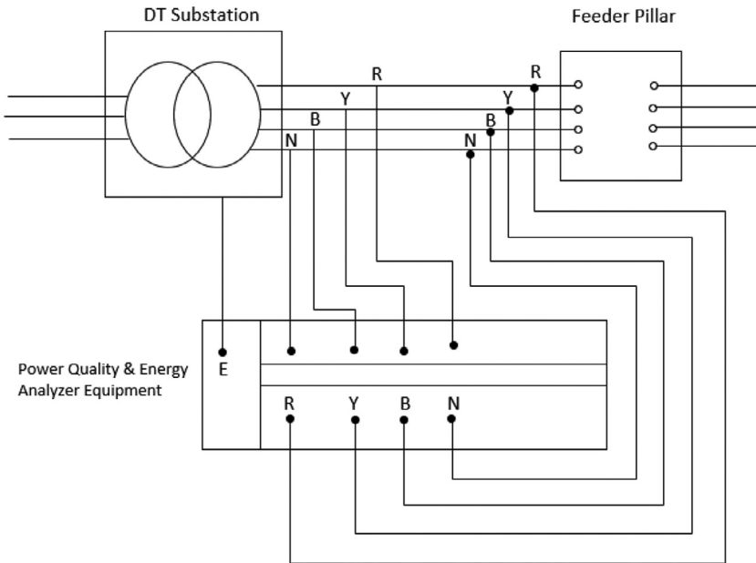
Fig. 1. Experimental circuit arrangement for substation operational management.
