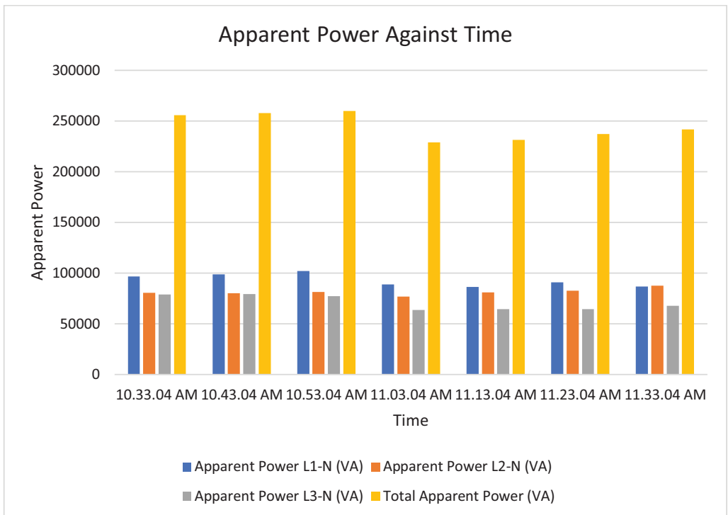
Fig. 16. Histogram representation of apparent power of each phase against Time.
