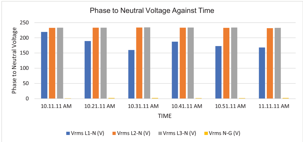
Fig. 3. Histogram representation of Vrms (Phase to Neutral) of each phase against Time.
