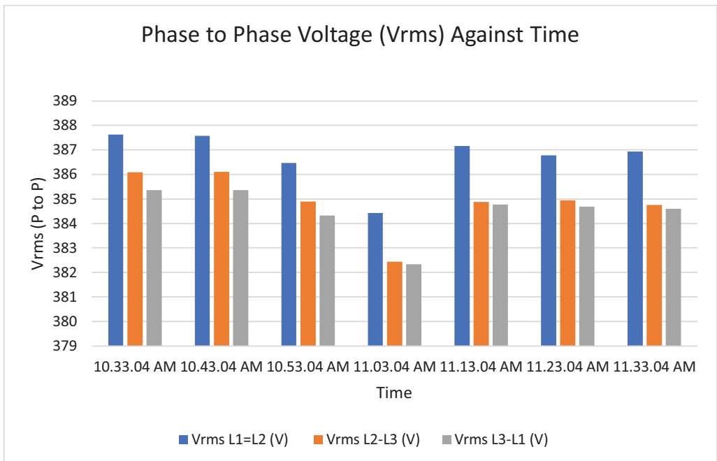
Fig. 12. Histogram representation of Vrms (Phase to Phase) against Time.
