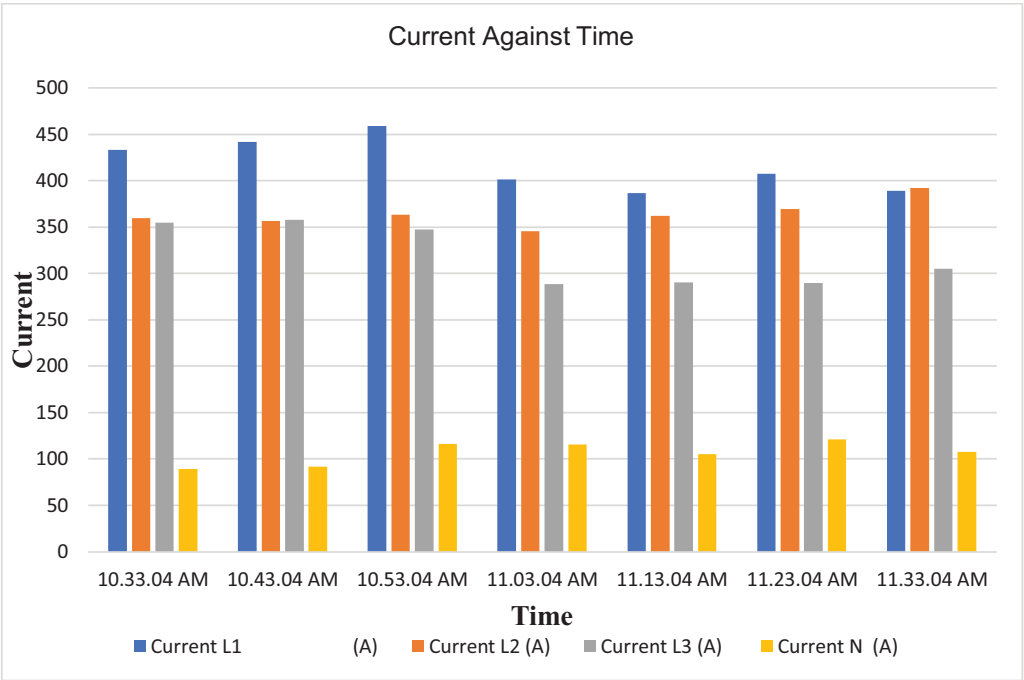
Fig. 13. Histogram representation of current of each phase against Time.
