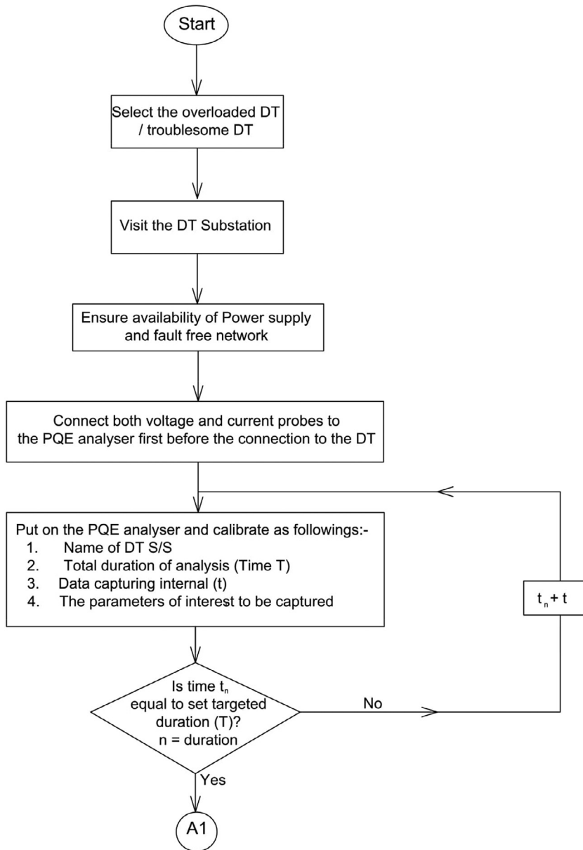
Fig. 2. (a) Flow process of typical DT power analysis using Power Quality and Energy Analyser Equipment. (b) Continuation of Flow process of typical DT power analysis using Power Quality and Energy Analyser Equipment.
