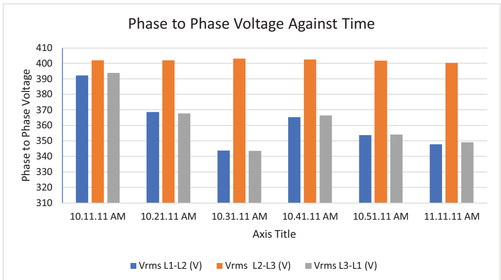
Fig. 4. Histogram representation of Vrms (Phase to Phase) against Time.
