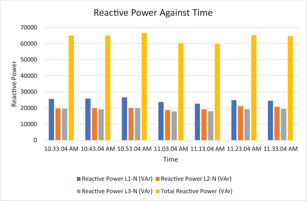
Fig. 17. Histogram representation of Reactive power of each phase against Time.
