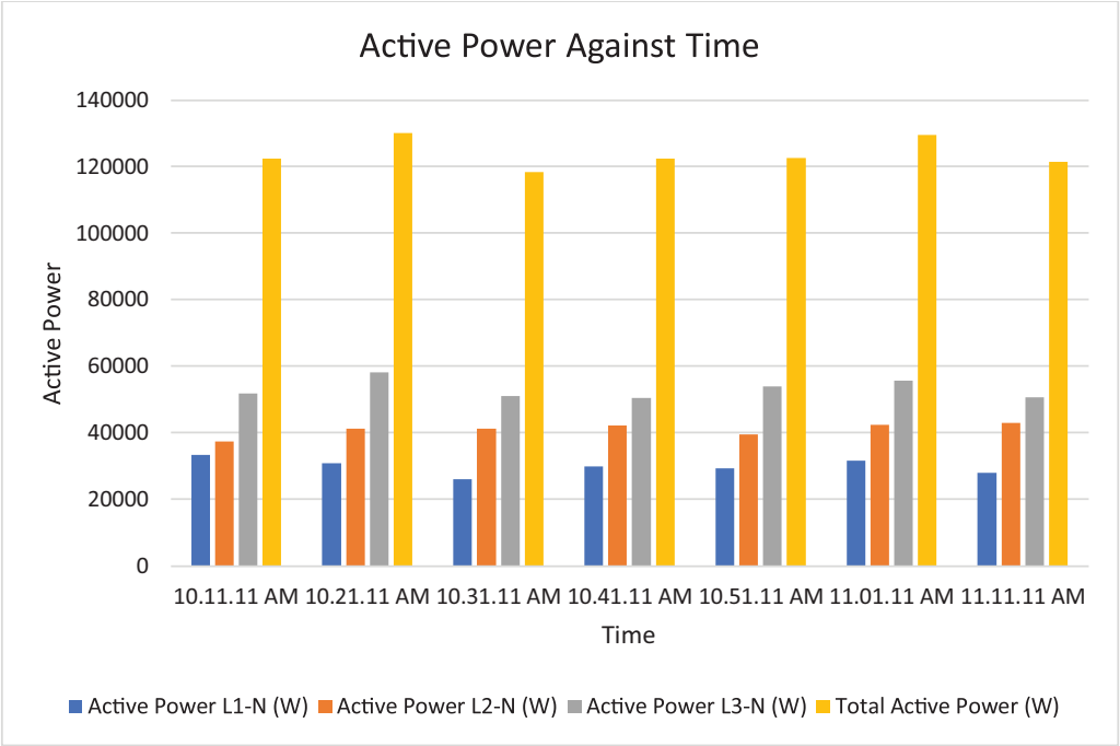
Fig. 9. Histogram representation of Active power of each phase against Time.
