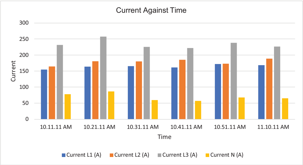
Fig. 5. Histogram representation of current of each phase against Time.
