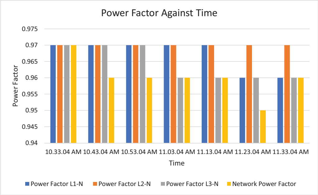
Fig. 18. Histogram representation of Power factor of each phase against Time.
