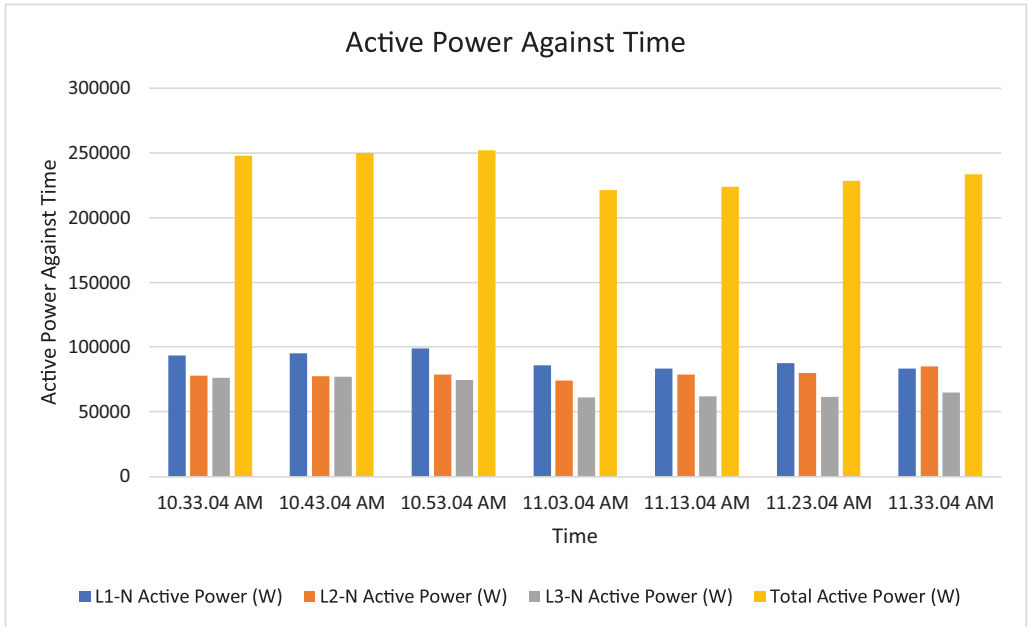
Fig. 15. Histogram representation of Active power of each phase against Time.
