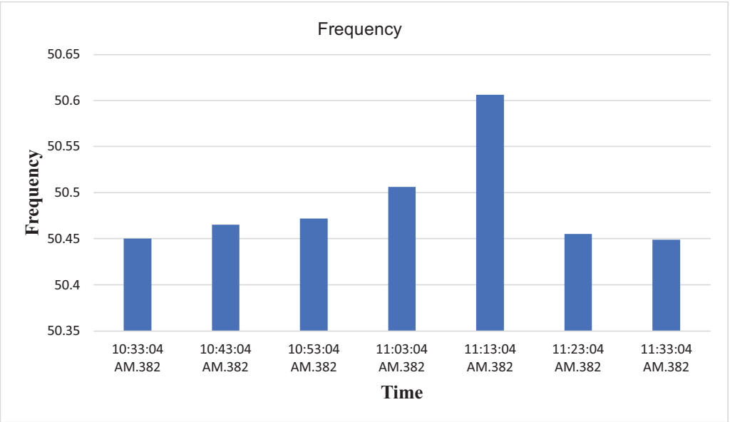
Fig. 14. Histogram representation of Frequency of each phase against Time.
