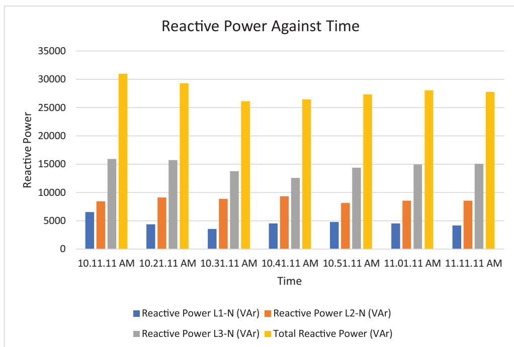
Fig. 8. Histogram representation of Reactive power of each phase against Time.
