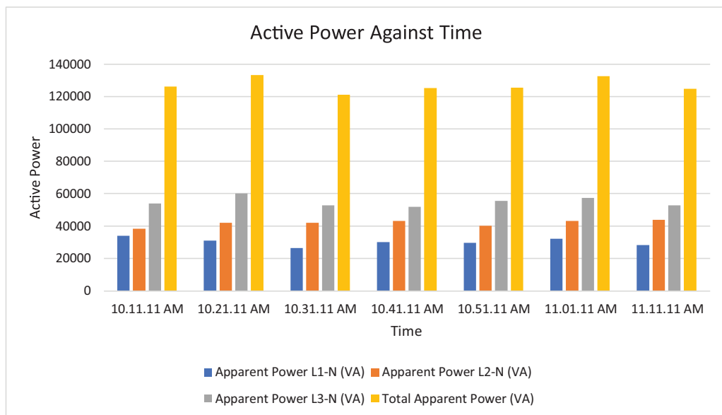
Fig. 7. Histogram representation of apparent power of each phase against Time.
