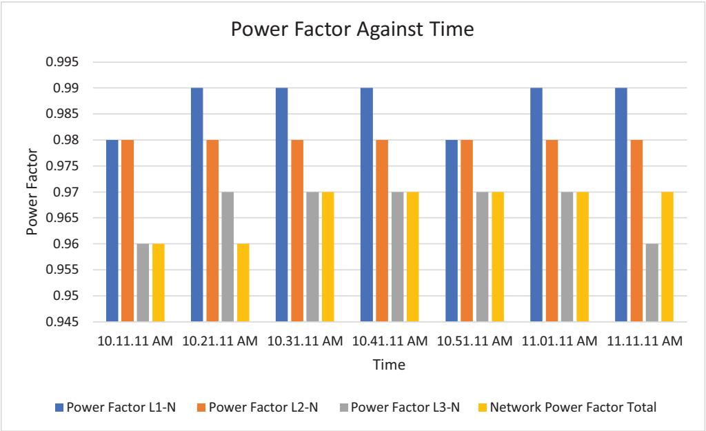
Fig. 10. Histogram representation of Power factor of each phase against Time.
