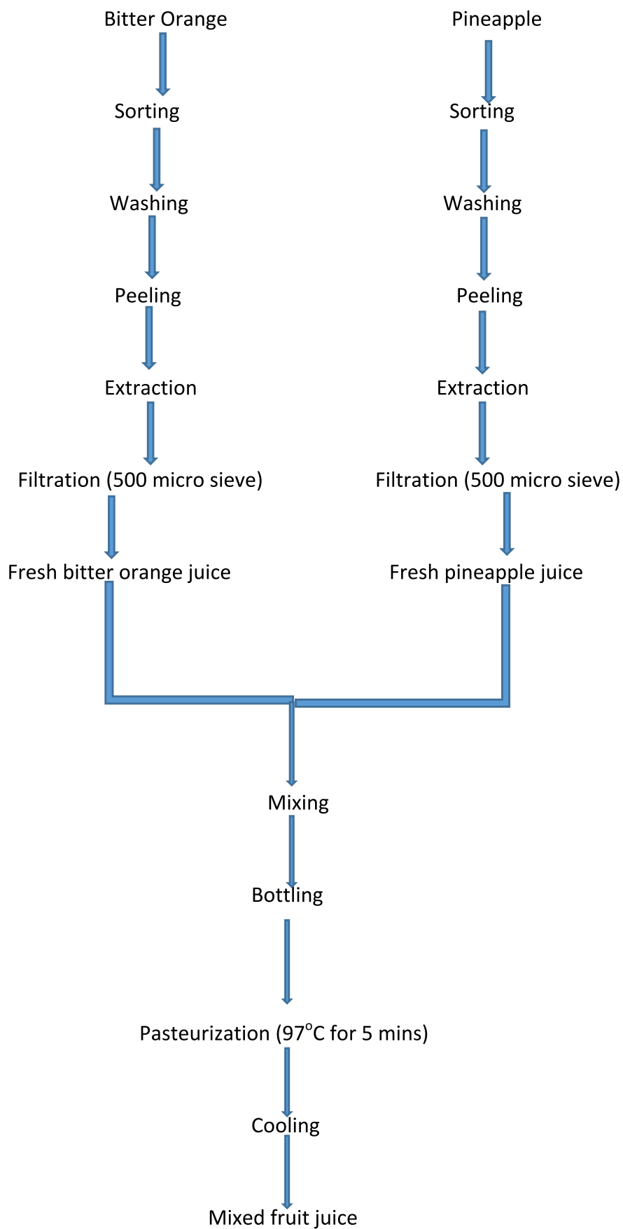
Fig. 1. Flow chart for the production of mixed fruit juice Source: Cemeroglu (2004).
