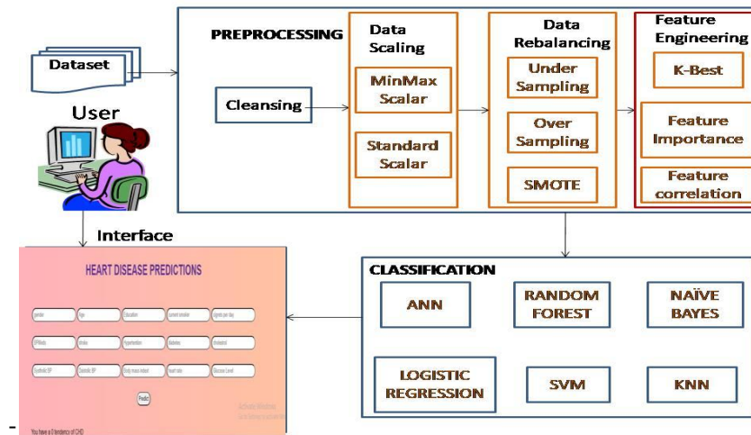
Fig. 2. Proposed heart disease predictive model
