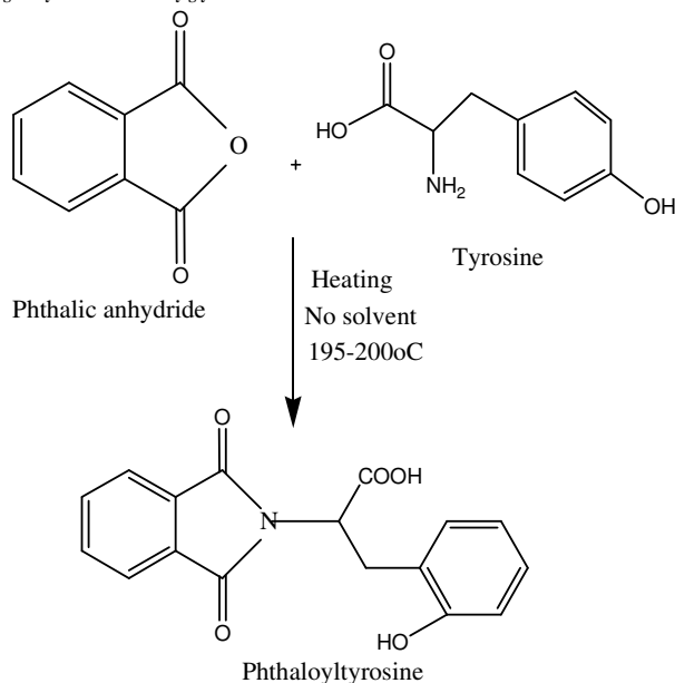
Fig.2: Synthesis of Phthaloyltyrosine
