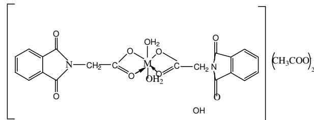
Fig.3: Proposed Structure of [\text{M}(\text{PHG})_2(\text{H}_2\text{O})_2](\text{CH}_3\text{COO})_2
