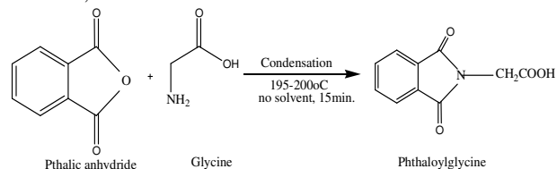
Fig. 1: Synthesis of Phthaloyltyrosine
