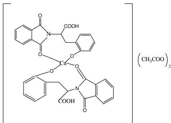
Fig.4: Proposed Structure of [\text{Cu}(\text{PHT})_2](\text{CH}_3\text{COO})_2
