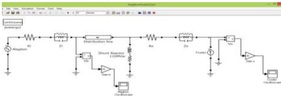
Figure 5: Developed Model Circuit of Alagbon – Alagbon Local Distribution Line for Harmonic Generation using MATLAB/Simulink simulation
