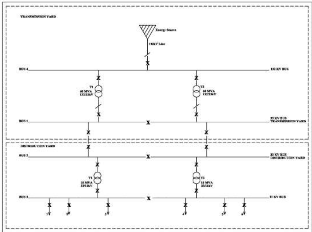
Figure 4: Typical 2 X 60 MVA 132/33kV Transmission yard at close proximity to 2 X 15 MVA 33/11kV Distribution Yard
