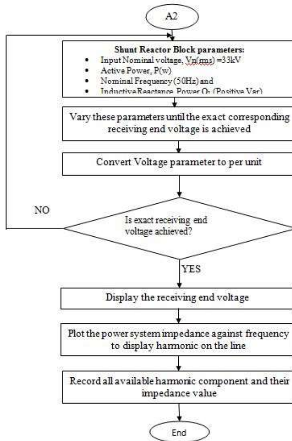
Figure 3: Development of Flow chart for harmonic evaluation on model TT Distribution line between two buses
