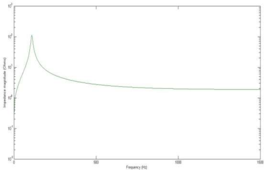
Figure 10: Harmonic on Alagbon – Alagbon Local Distribution Line at 06:00Hrs
